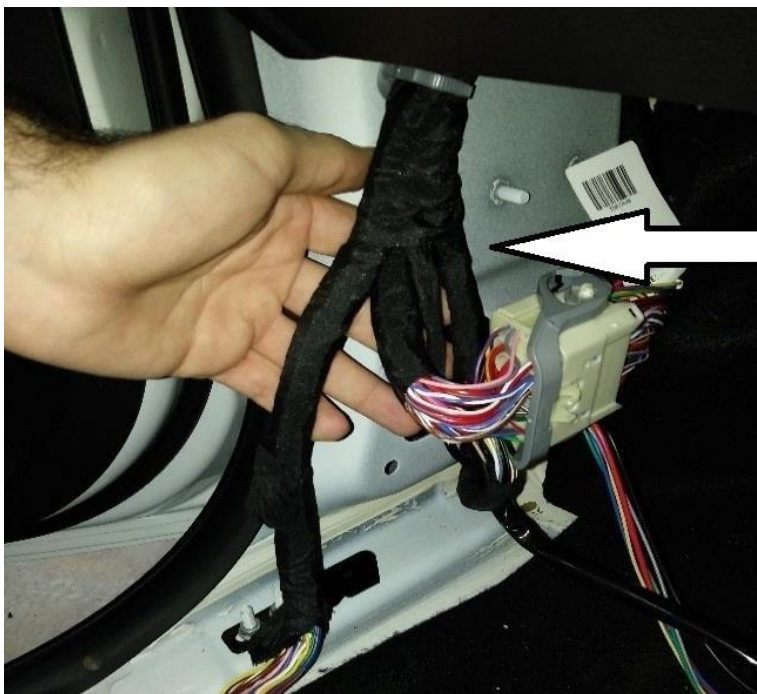
Harness for Lock & Unlock Signal
